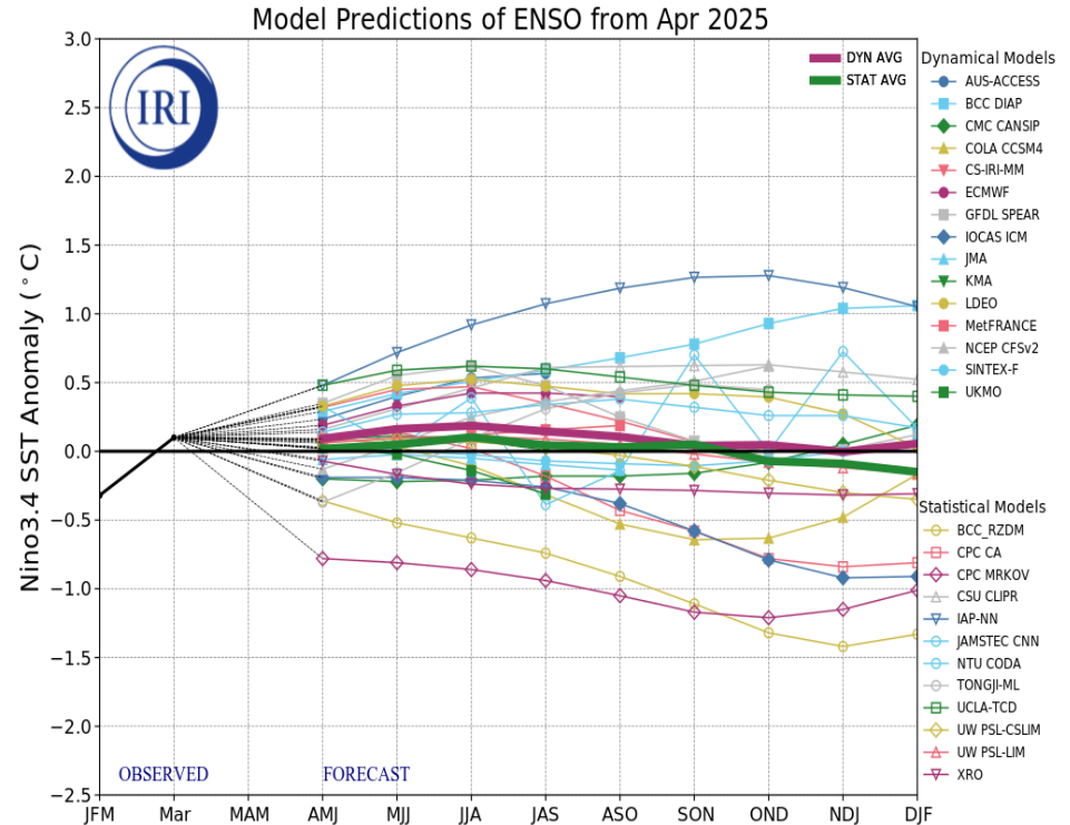
Figure provided by the International Research Institute (IRI) for Climate and Society (updated 21 April 2025).
